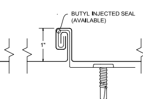
180° SEAM DETAIL
