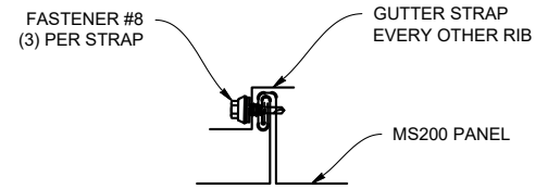
GUTTER STRAP ATTACHMENT
