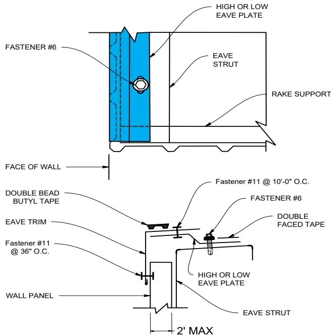
WALL PANEL INSTALLED BEFORE ROOF
