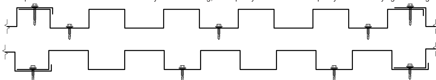
PANEL ATTACHMENT
