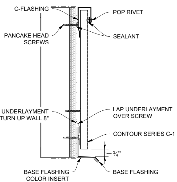
DOOR/WINDOW HEAD DETAIL: VERTICAL PANEL
