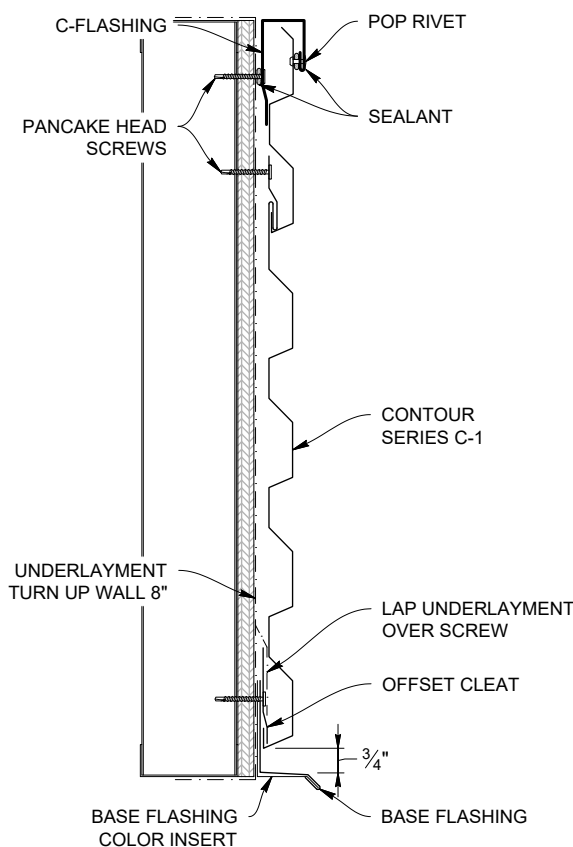
DOOR/WINDOW HEAD DETAIL: HORIZONTAL PANEL
