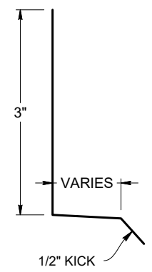
PART SHOWN: CONTOUR OFFSET CLEAT
