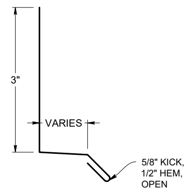
PART SHOWN: CONTOUR C-FLASHING
