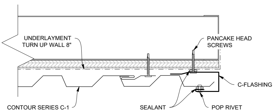
DOOR/WINDOW JAMB DETAIL: VERTICAL PANEL
