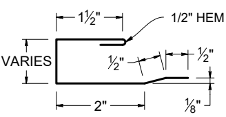
PART SHOWN: CONTOUR C-FLASHING
