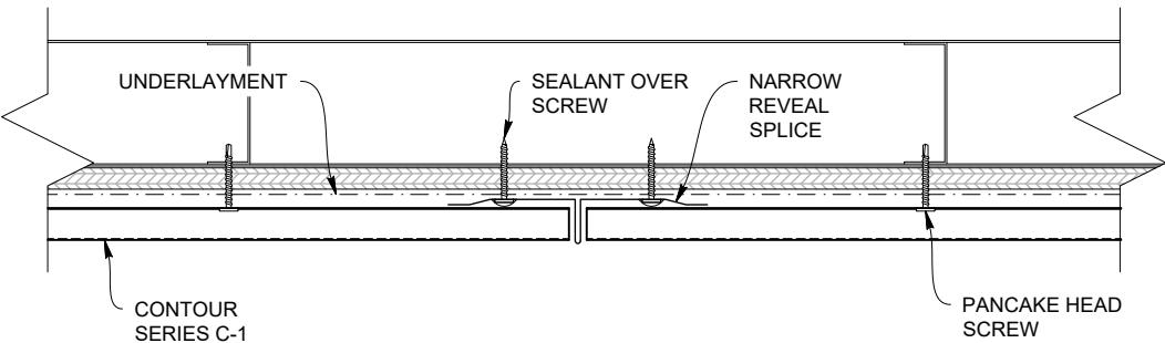
NARROW REVEAL SPLICE DETAIL
