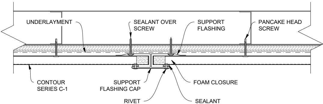
SUPPORT FLASHING CAP DETAIL
