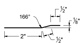
PART SHOWN: CONTOUR OFFSET CLEAT
