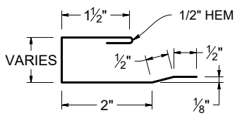
PART SHOWN: CONTOUR C-FLASHING
