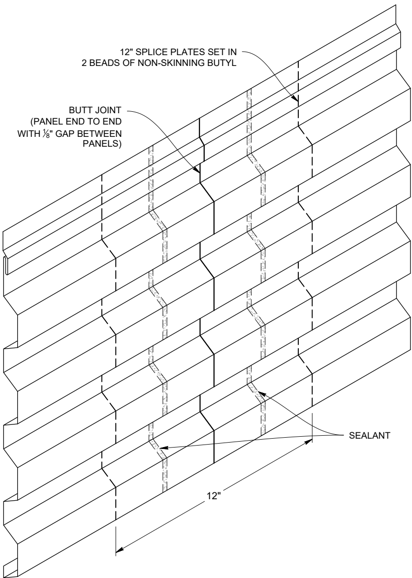
Panel Lap 2: C-1 Panel Shown
