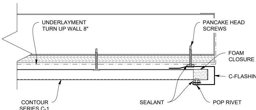
DOOR/WINDOW JAMB DETAIL: HORIZONTAL PANEL
