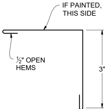
OUTSIDE CORNER - TYPE A - STANDARD CLIP / SCREW ( TKCTCOAS ) FLANGE
