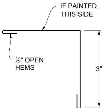
OUTSIDE CORNER - TYPE A - STANDOFF CLIP (TKCTCOAS)
