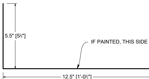
5-1/2" PAN FLASHING (SLP5)
