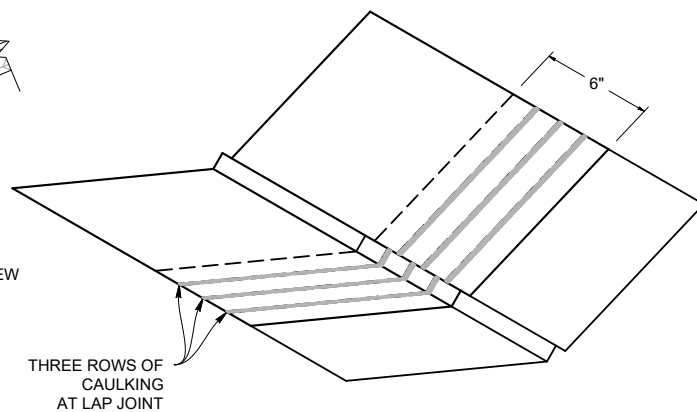
VALLEY LAP
