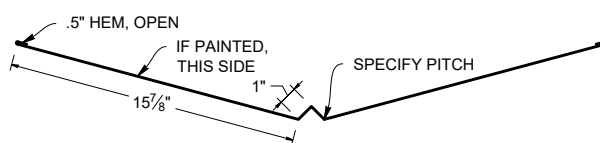
VALLEY LAP
