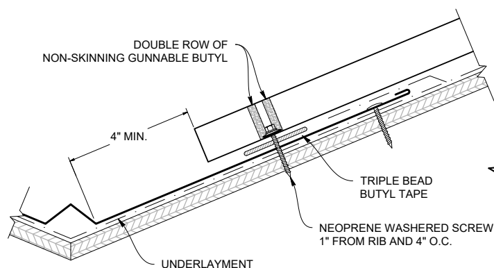
ALTERNATE VALLEY FLASHING DETAIL (Less Than 3:12 Pitch - Not Recommended)
