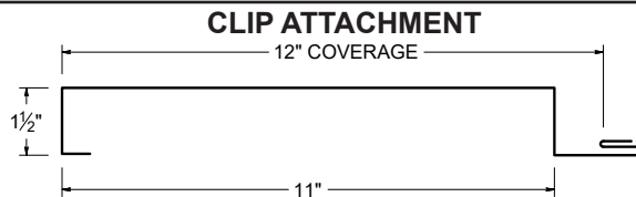
STANDARD CLIP
