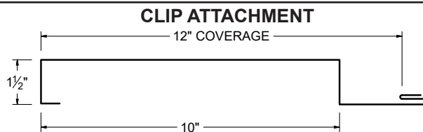
STANDARD CLIP
