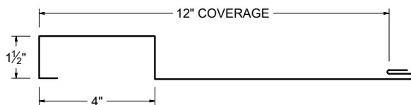
STANDARD CLIP
