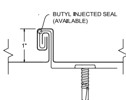
180° SEAM DETAIL
