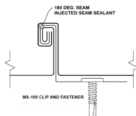
180° Seam
