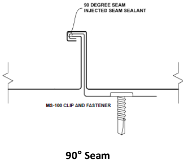
90° Seam
