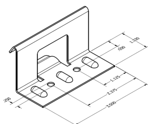
Versa-Span Snap-Lock Clip
