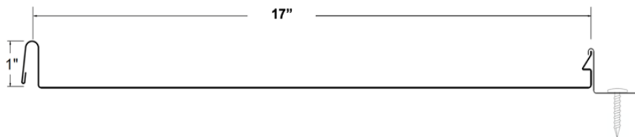
Roofing Panel Profile and Typical Installation
