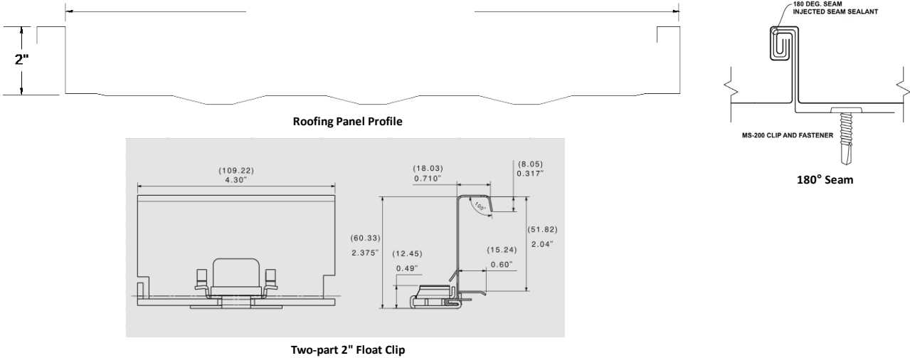
FIGURE 7—MS-200 PANELS - 180° PANEL SEAM
