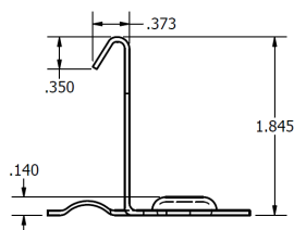
FIGURE 11—VERSA-SPAN PANEL
