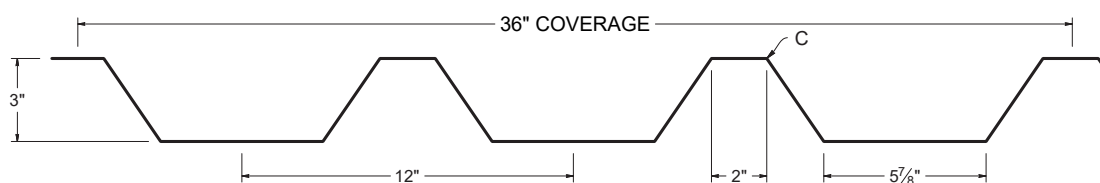
36" Single Lap Coverage
