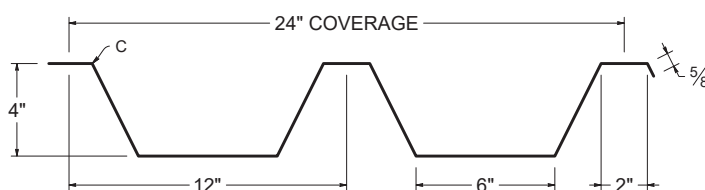
24" Single Lap Coverage
