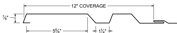
SCREW FLANGE ATTACHMENT
