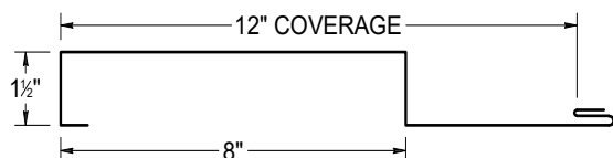
CLIP ATTACHMENT
