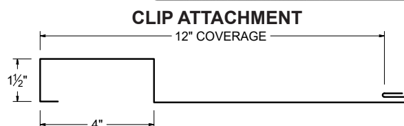
STANDARD CLIP
