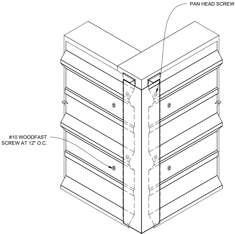
PART SHOWN: (T3CPO) .75" OUTSIDE CORNER POST
