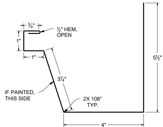
BOX GUTTER ( T3BG )
