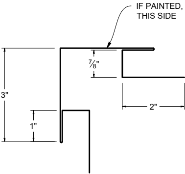
PART SHOWN: (T3CPO) .75" OUTSIDE CORNER POST
