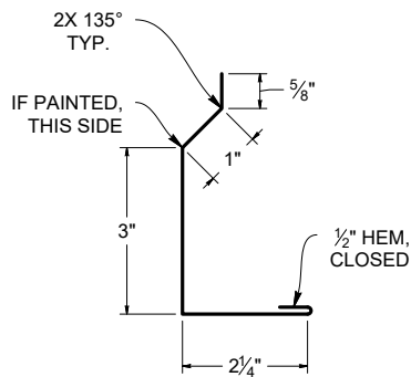
.75" DOOR RAIL COVER ( T3DRC )
