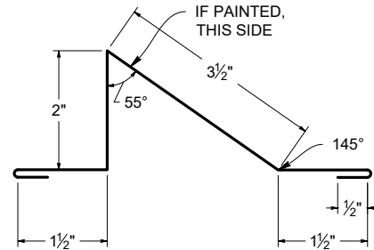
.75 RSP SNOW BREAK ( T3RSB )
