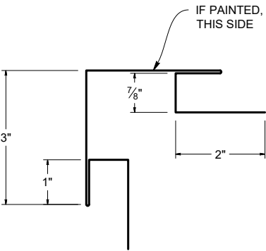
PART SHOWN: (T3CPO) .75" OUTSIDE CORNER POST
