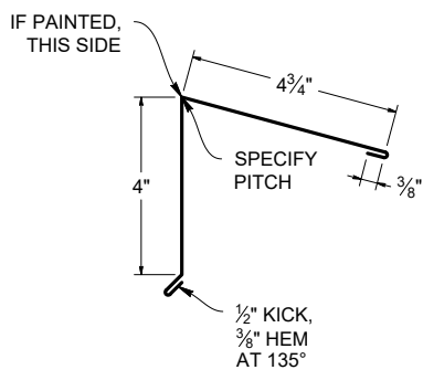
4" PEAK CAP ( T3RP4)
