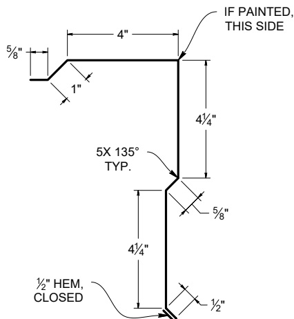
.75" 2X8 STEP GABLE ( T3SG8 )
