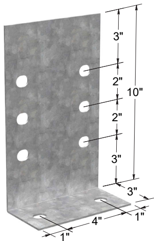
10" x 3" Purlin Clip
