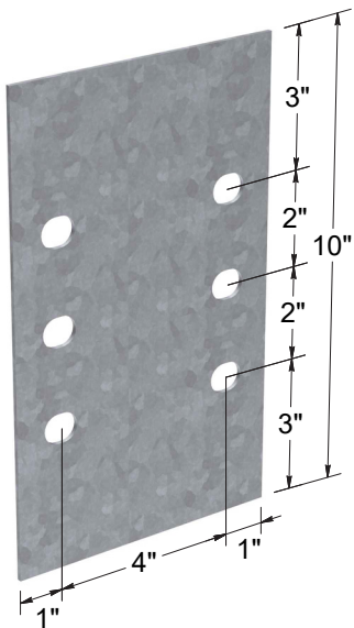
10" x 6" Purlin Clip
