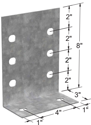
8" x 3" Purlin Clip
