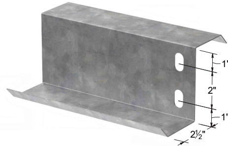
4" x 2.5" Zee
