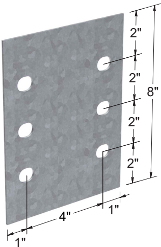
8" x 6" Purlin Clip
