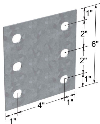
6" x 6" Purlin Clip
