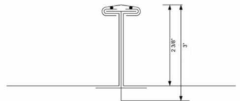
AFTER SEAMING
