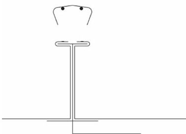
SEAM ENGAGEMENT
