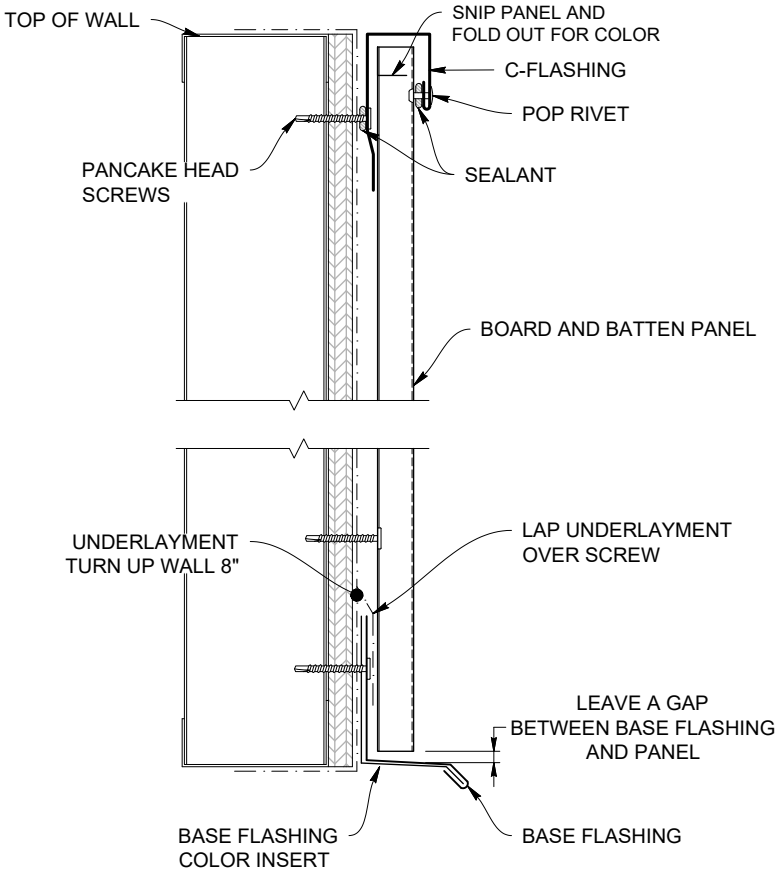
BASE FLASHING DETAIL: HORIZONTAL
