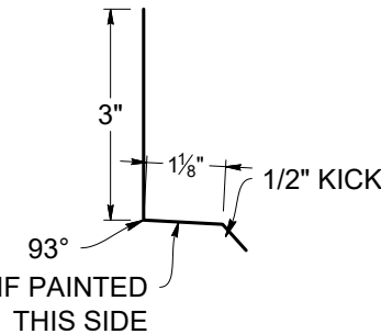
PART SHOWN: BASE FLASHING INSERT PART NUMBER BBBFI
