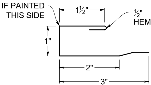
PART SHOWN: C-METAL PART NUMBER: BBCF
